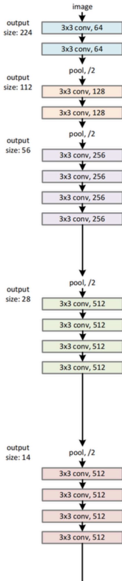
VGG-19
