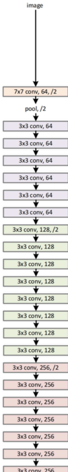
34-layer plain
